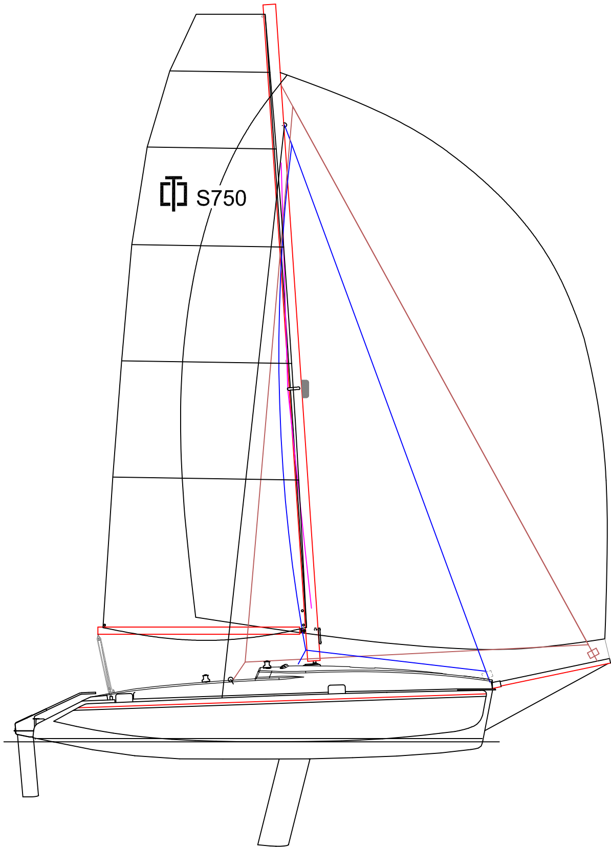
SPRINT 750 MKII SAILPLAN
